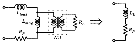
Figure 3: Simplified Load Model
