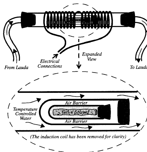
Figure 2: Close-up of Solenoid/Gel Assembly
