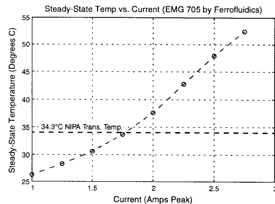
Figure 10: Ferrofluid Equilibrium Temp. vs. Current
