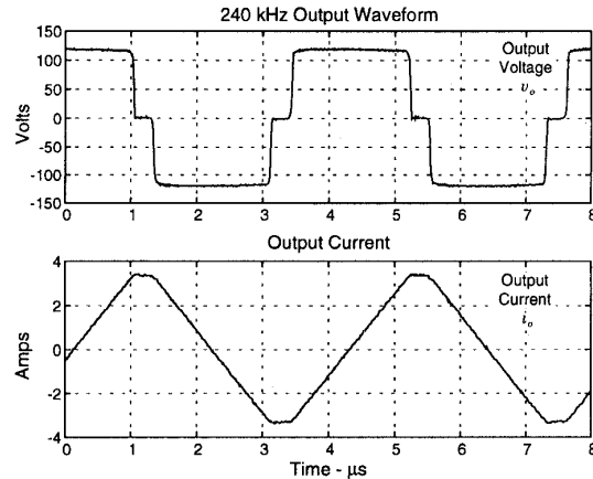
Figure 5: ZVS Full-Bridge Waveforms
