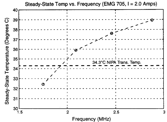
Figure 11: Ferrofluid Equilibrium Temp. vs. Frequency
