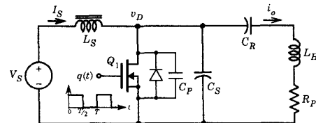
Figure 6: Class E Schematic
