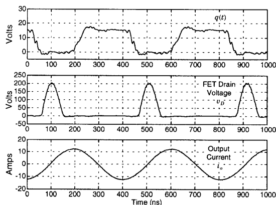
Figure 7: 2.5MHz Class E Waveforms
