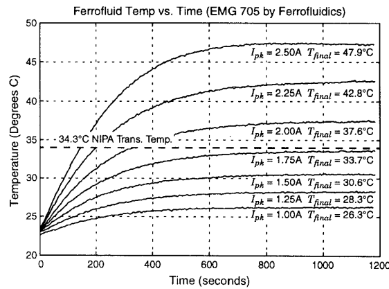
Figure 9: Ferrofluid Temperature vs. Time
