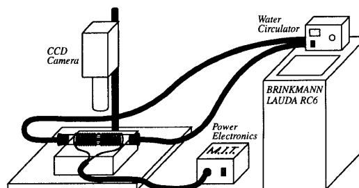
Figure 1: Experimental Setup
