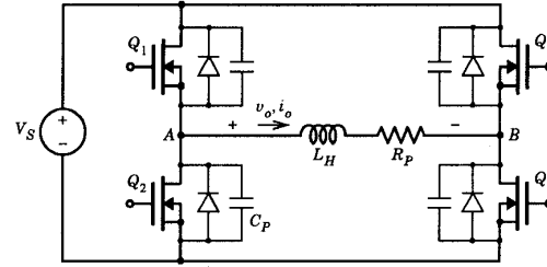
Figure 4: ZVS Full-Bridge Schematic
