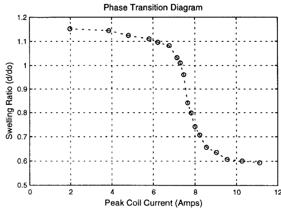
Figure 8: Phase Transition Curve
