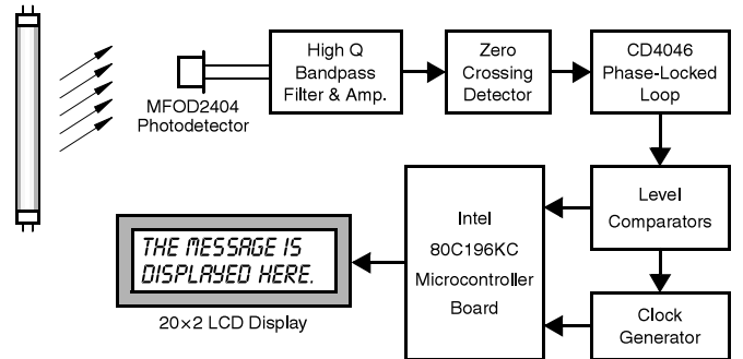
Fig. 6. Receiver block diagram.
