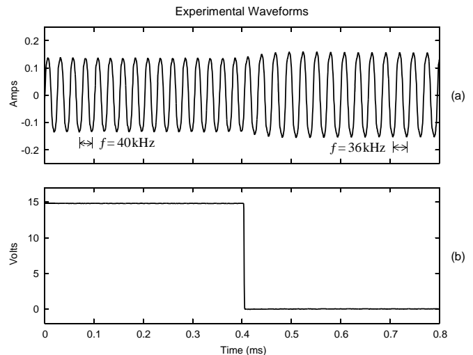
Fig. 10. Expanded view of the lamp current during a step change in frequency.
