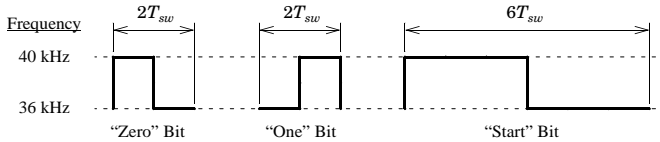
Fig. 3. Manchester bit patterns.
