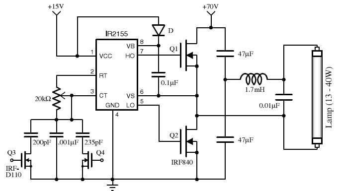
Fig. 1. Lamp ballast circuit.
