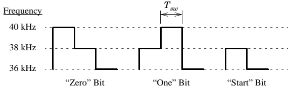
Fig. 2. Three-level bit patterns.
