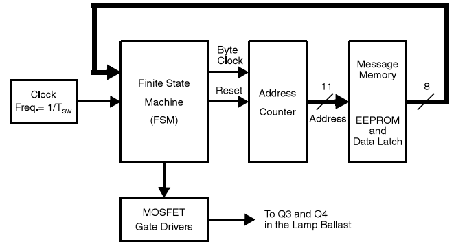
Fig. 5. Transmitter block diagram.
