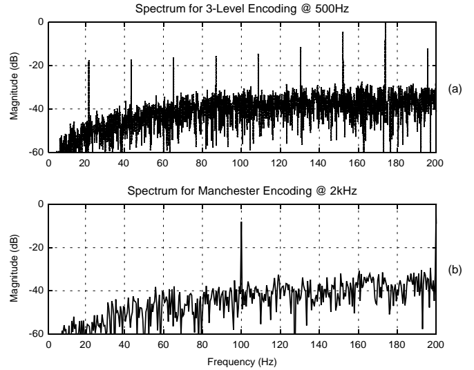
Fig. 4. Predicted frequency spectrum of lamp intensity.
