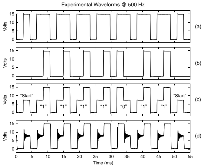
Fig. 7. Transmitted and received bit patterns with 3-level encoding.
