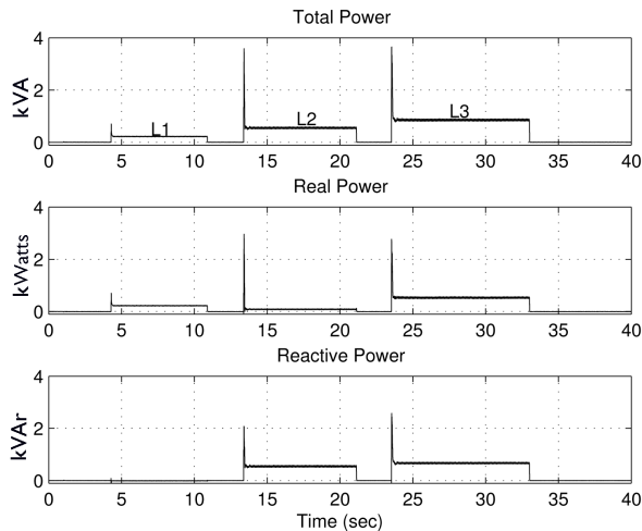
Fig. 8. Total, real and reactive power draw
