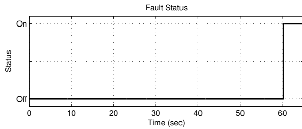
Fig. 16. Shunt trip signal for adaptive MFM
