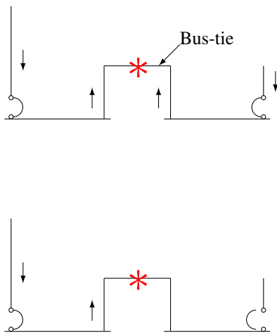
Fig. 4. Examples of bus-tie faults.
