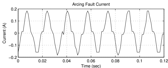
Fig. 17. Arcing fault current
