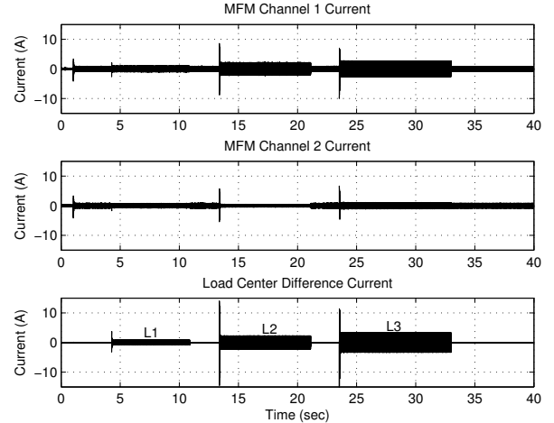
Fig. 7. MFM currents
