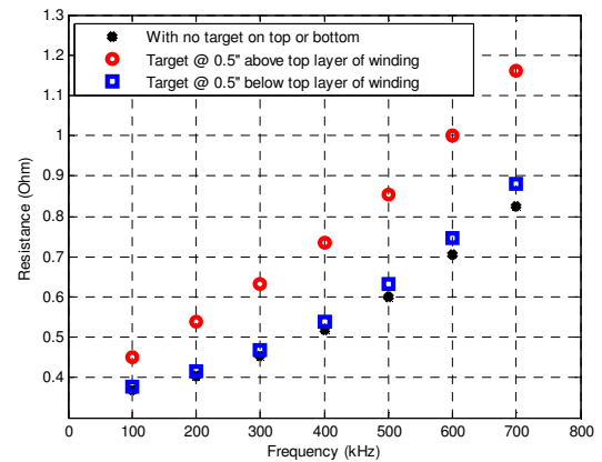
Figure 11. Measurement data from impedance analyzer: Change in resistance when a target is placed above the top layer winding is significantly higher compared to the change when the target is placed at same distance below.
