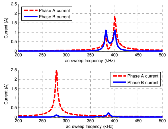
Figure 9. SPICE ac sweep result: Effect of stray coupling on B-phase with only A-phase excited. Top: Both phases tuned at 400 kHz. Significant current induced in the B-phase at same frequency. Bottom: A-Phase is tuned at 280 kHz while B-phase is tuned at 387 kHz. Cross-coupling effect is significantly reduced.
