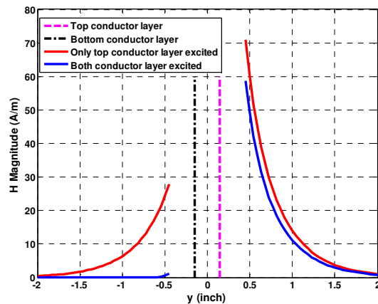
Figure 4. Rapid roll-off of the magnetic field on the bottom of the cell compared to the top in the presence of the bottom conductor layer at x=0 .
