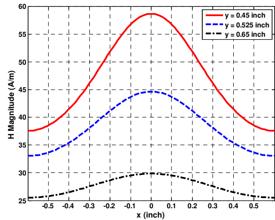
Figure 3. Near-sinusoidal variation of the magnetic field along x -direction for the optimized Halbach conductor arrangement using six conductors.
