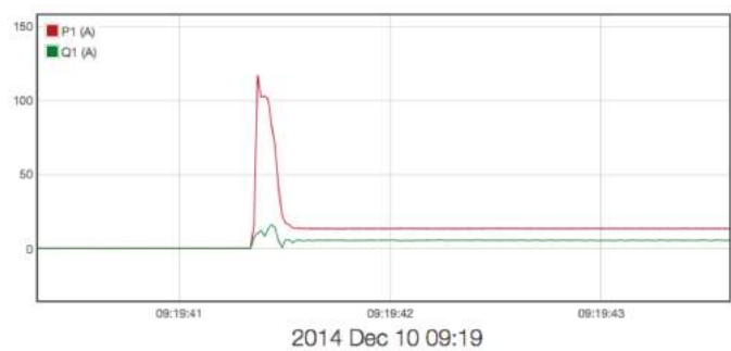
Figure 15. Startup transient for CPP pump.
