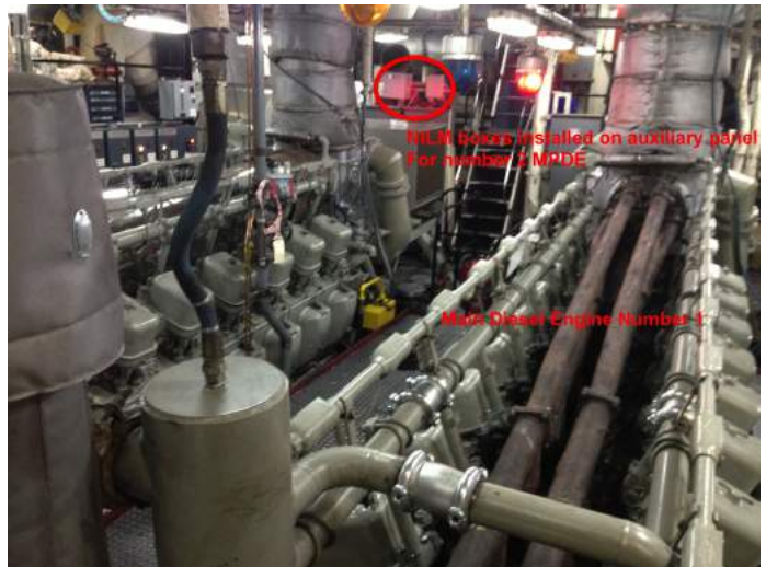
Figure 4. USCGC SPENCER engine room. Nonintrusive monitors are installed forward of the #2 MPDE just above the monitored panel.
