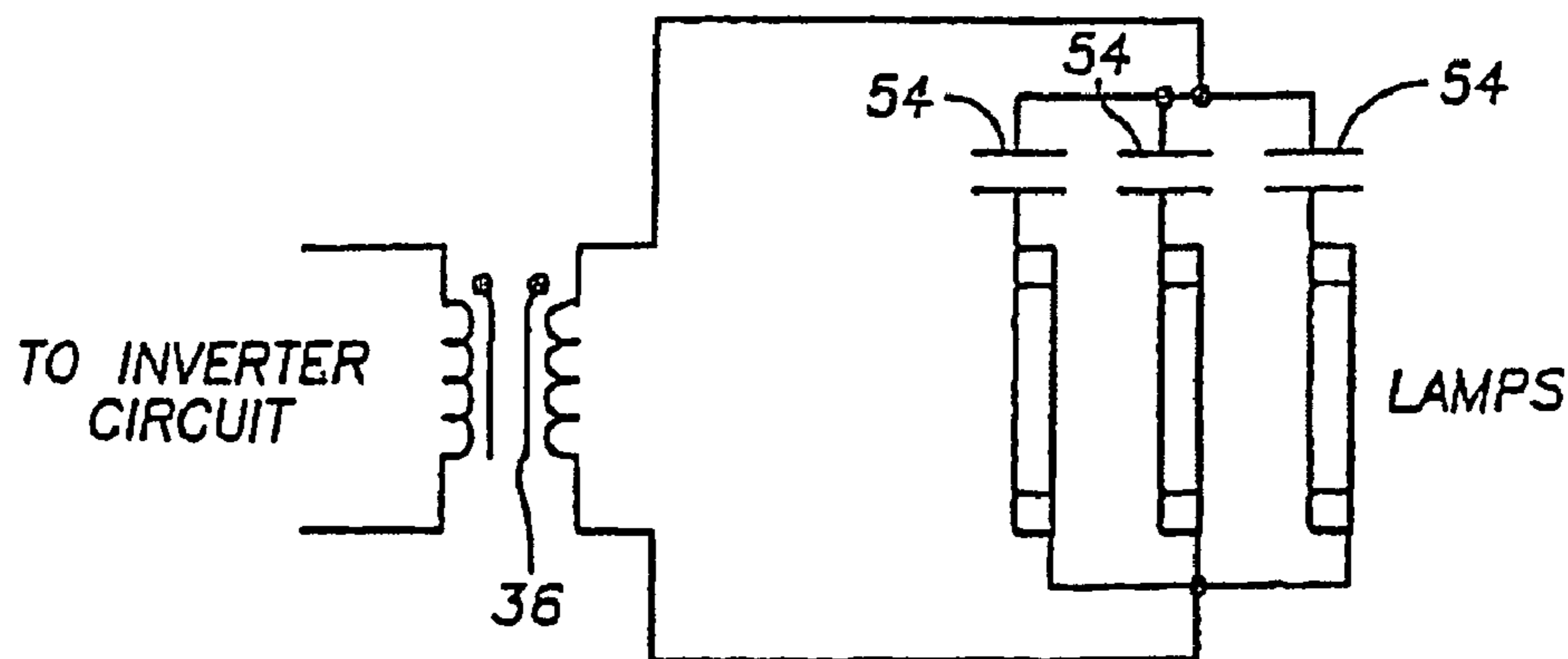
FIG. 6c SAMPLE LOAD CONFIGURATIONS.
