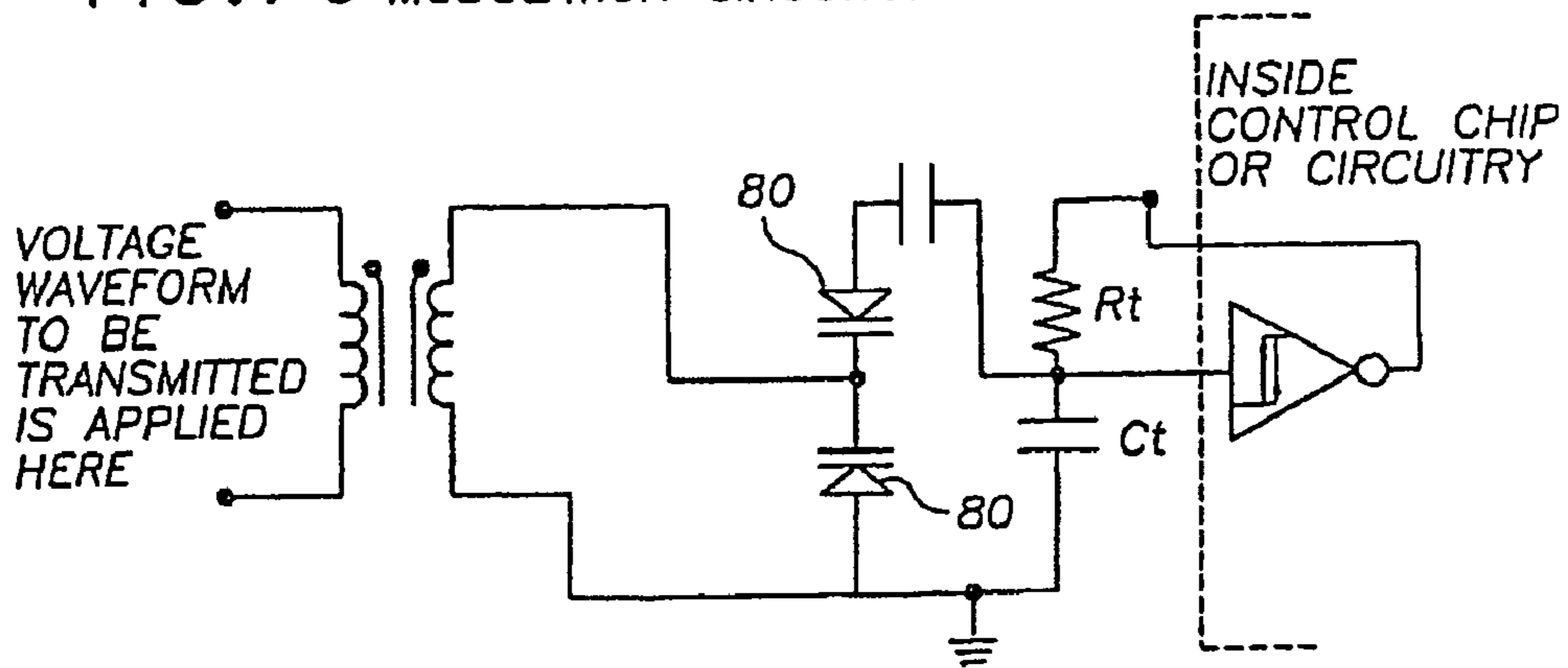
FIG. 7c MODULATION CIRCUITS.
