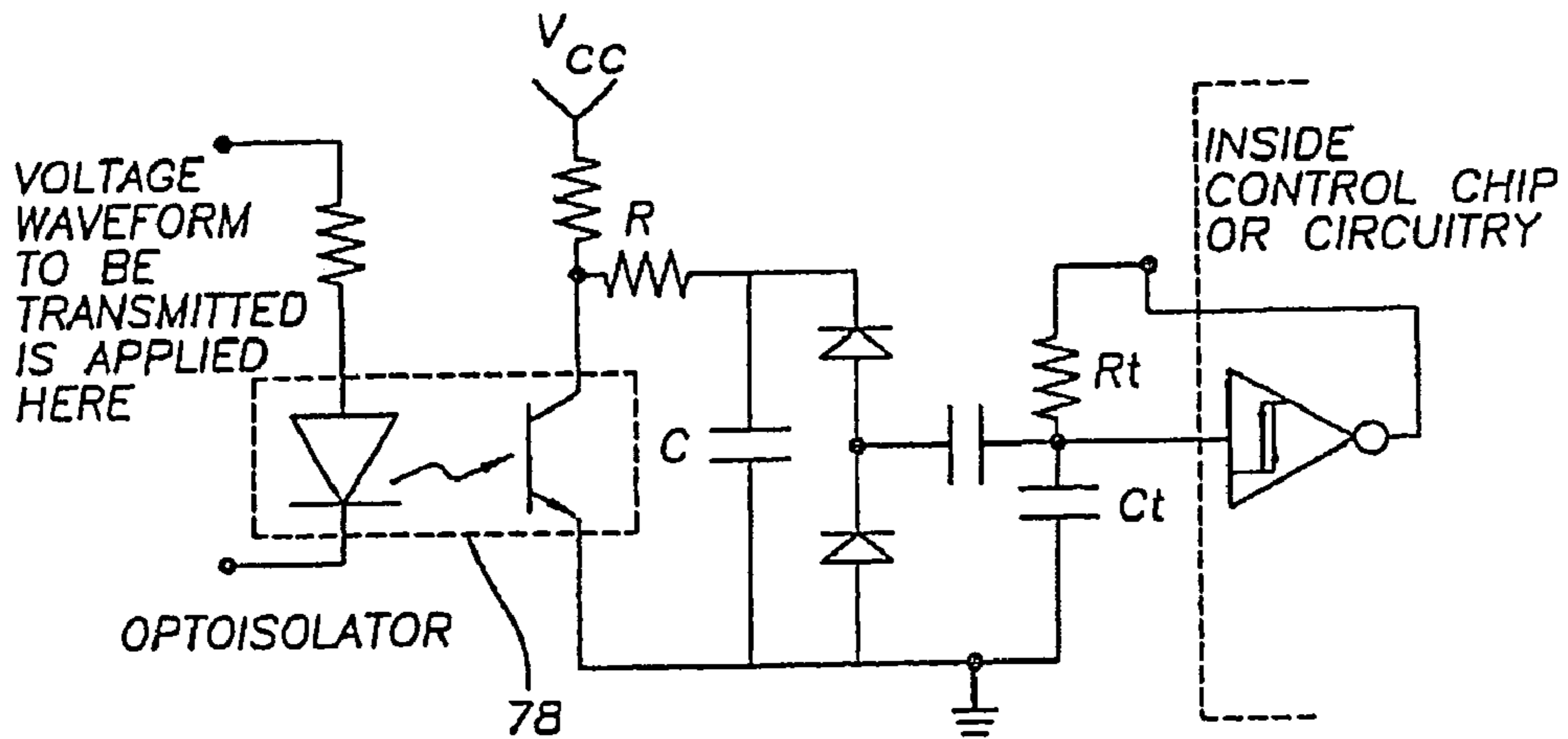
FIG. 7b MODULATION CIRCUITS.
