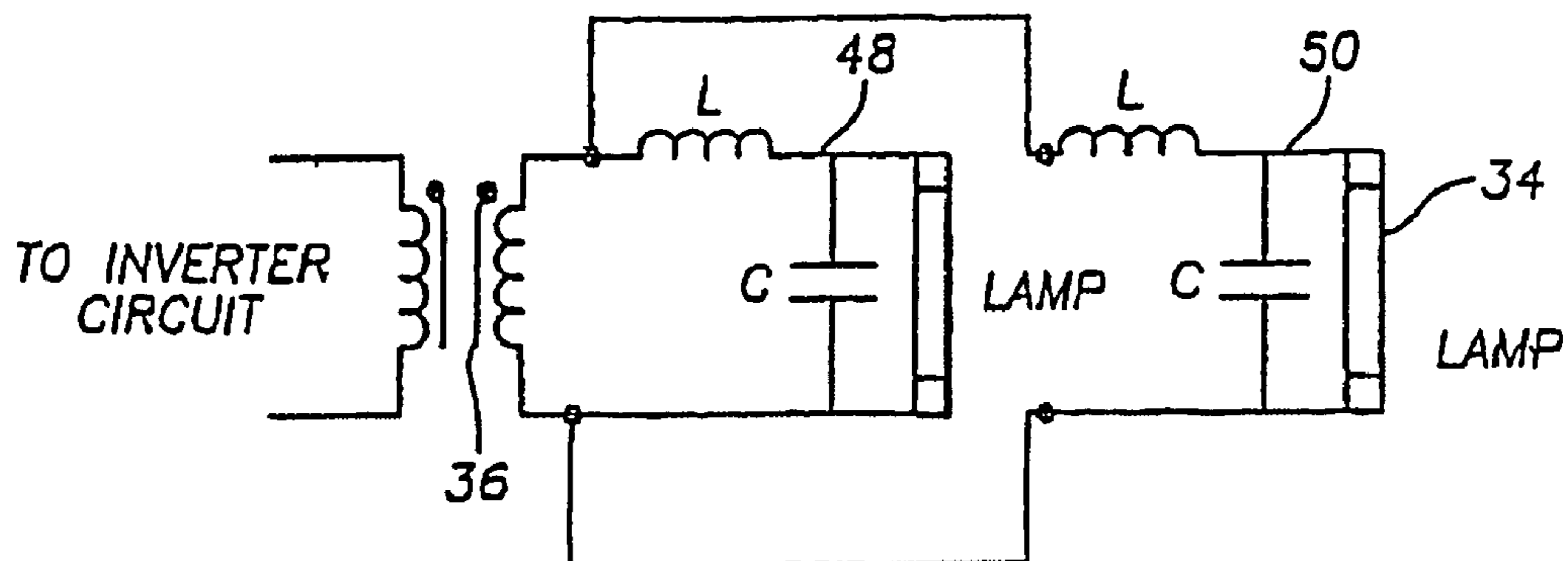
FIG. 6a SAMPLE LOAD CONFIGURATIONS.
