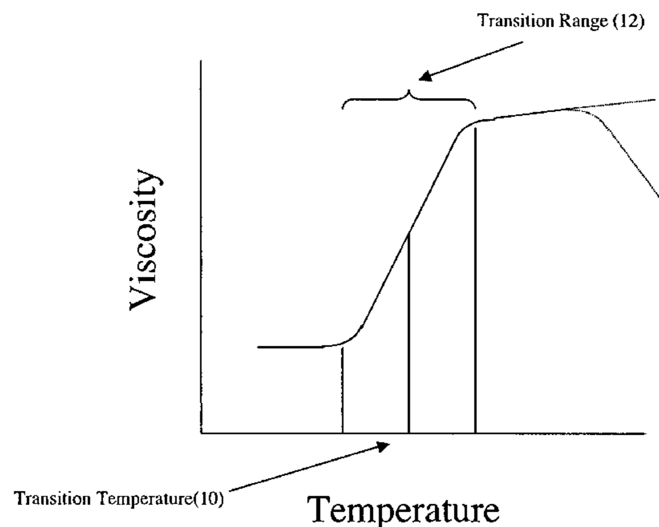
Viscosity/Temperature Curve for a Reverse Thermal Fluid
