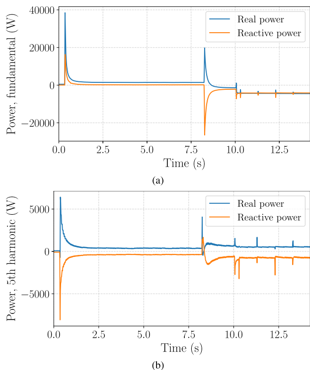
FIGURE 13. a) Sum of the three phases of the real and reactive power of a shipboard VFD operating at the a) fundamental frequency, b) fifth harmonic component.
