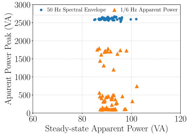
FIGURE 5. Scatter plot comparison of fridge events’ peak and steady-state apparent powers, for both the 50 Hz (blue cluster) and 1/6 Hz UK-DALE data (orange cluster). The spectral envelope cluster shows less variability in apparent power peak (std dev = 29.11 VA) compared to the 1/6 Hz cluster (std dev = 611.40 VA).
