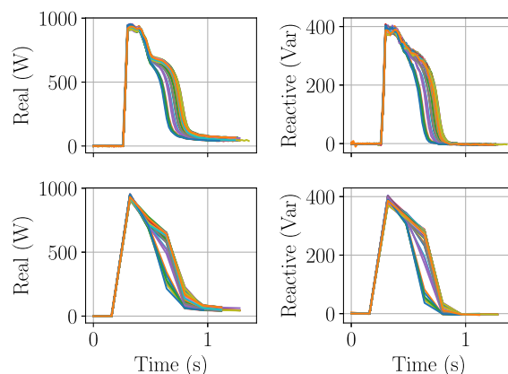
FIGURE 15. Real and reactive power transients for fridge on events. The top row has a data rate of 50 Hz, and the bottom row is downsampled by a factor of 8. Downsampling smooths the transient shape and reduces apparent between-event variability.
