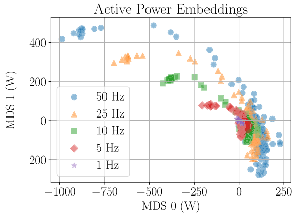
FIGURE 16. Multidimensional scaling (MDS) embeddings of the real power fridge on transients across multiple sampling rates. As the sampling rate decreases, the embeddings collapse toward a tight cluster, indicating loss of transient-shape information and reduced feature-space separability.
