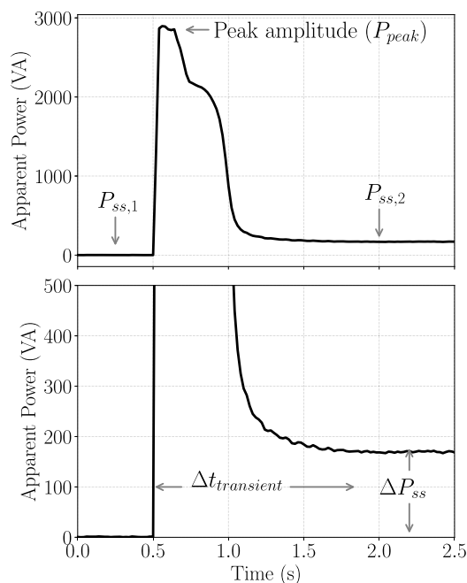
FIGURE 3. Transient features such as peak amplitude ( P_{peak} ), shape, steady-state levels ( P_{ss,1} and P_{ss,2} ) (top figure), and transient duration ( \Delta t_{transient} ) (bottom figure) are useful for geometric event identification. Additionally, these features also provide physical insights for electric machine diagnostics and fault detection.
